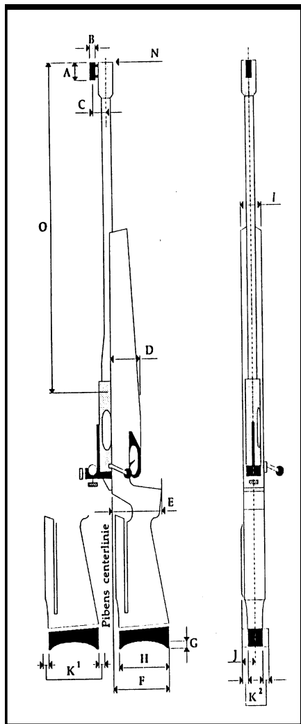
Figur 1: Biathlonriffel cal. 22
